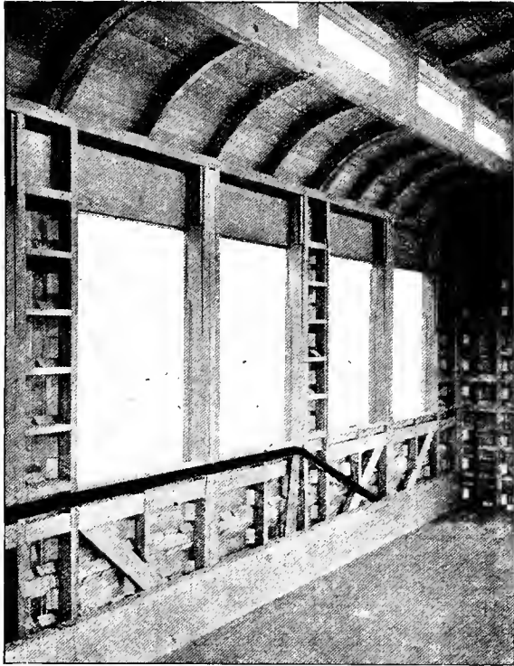
Fig. 532. Interior View, showing Blocking and Overhang Truss-rod and Strut.
